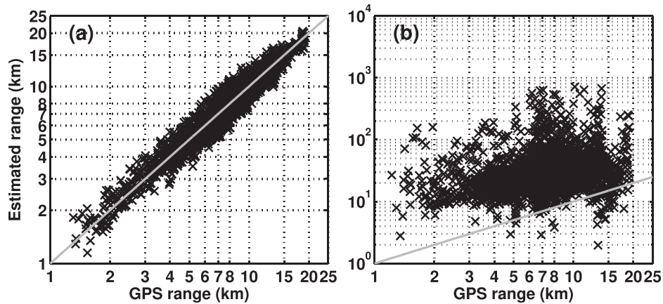
FIG. 9. A total of 2547 controlled source transmissions of 0.6- or 1-s broadband LFM non-impulsive signals with 50 Hz bandwidth are used to quantify the rms error of source range estimation by the generalized array invariant method with nonlinear matched filtering and without any matched filtering. (a) With nonlinear matched filtering, the source range estimates \hat{\rho}_0 of the vertical source array are plotted in logarithmic scale against GPS measured source range \rho_0 for the source range between 1 and 20 km and the source bearing between 0^\circ and 80^\circ from the receiver array endfire direction. The rms error of all range estimates is roughly 12% of the GPS measured source range. The solid gray line indicates the true source range measured by GPS. (b) Without any matched filtering, the error on average is roughly 800% of the GPS measured source range. Here, the solid black line also indicates the true source range measured by GPS. By comparing the range estimation results shown in (a) and (b), it highlights the need for pulse compression of the kind enabled by nonlinear matched filtering to improve the source localization accuracy for non-impulsive signals whose modal arrivals may not be otherwise resolvable.
